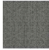
FLANNEL
